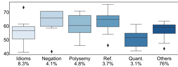
Figure 4: Categorized accuracy in for MCP(XLNet-R L ) on X-CODAH. Each box is for 15 languages.
